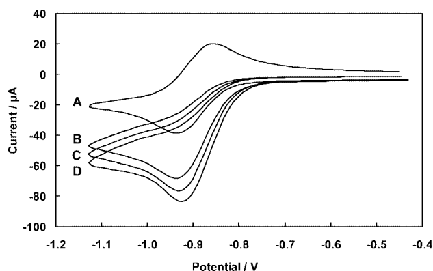
Figure 2. Cyclic voltammograms recorded with a glassy carbon disk electrode (area = 0.077 \text{ cm}^2 ) at 100 \text{ mVs}^{-1} in air-free DMF containing 0.10 \text{ M} \text{TMABF}_4 and (A) 2.0 \text{ mM} nickel(II) salen, (B) 2.0 \text{ mM} nickel(II) salen and 5.0 \text{ mM} 7-bromo-1-phenyl-1-heptyne, (C) 2.0 \text{ mM} nickel(II) salen and 10.0 \text{ mM} 7-bromo-1-phenyl-1-heptyne, and (D) 2.0 \text{ mM} nickel(II) salen and 20.0 \text{ mM} 7-bromo-1-phenyl-1-heptyne. Scans go from -0.45 to -1.13 to -0.45 V.
